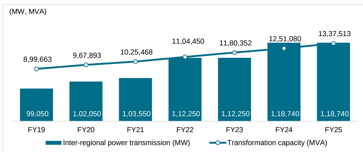
Figure 19: Growth in transformation capacity and inter-regional power transmission capacity
