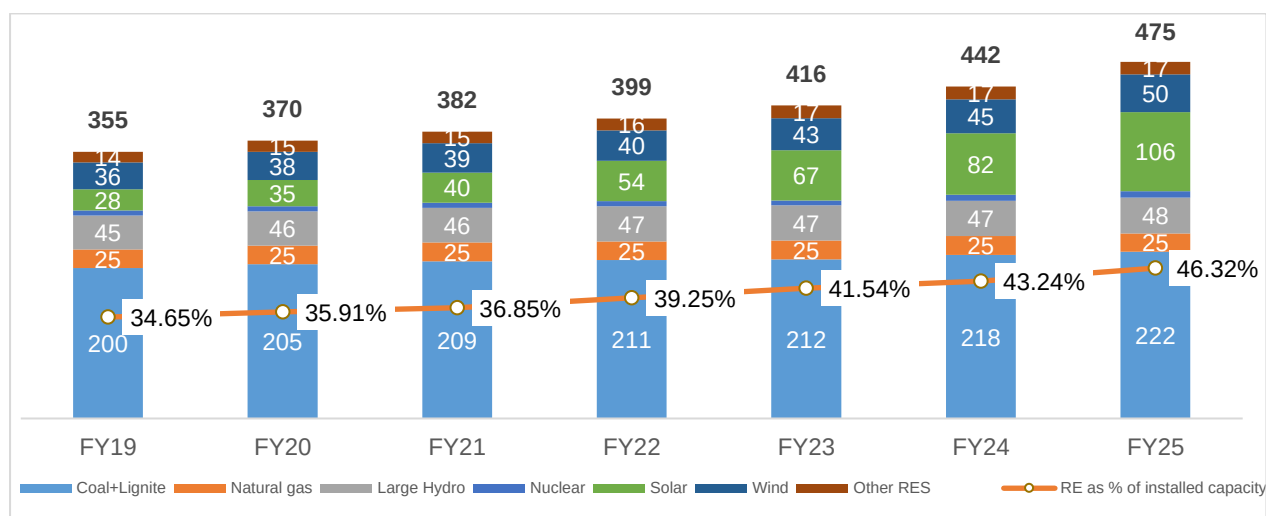
Figure 11: Historical Fuel-wise installed capacity (GW)
