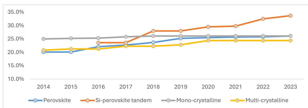
Figure 33: Cell efficiency comparison
